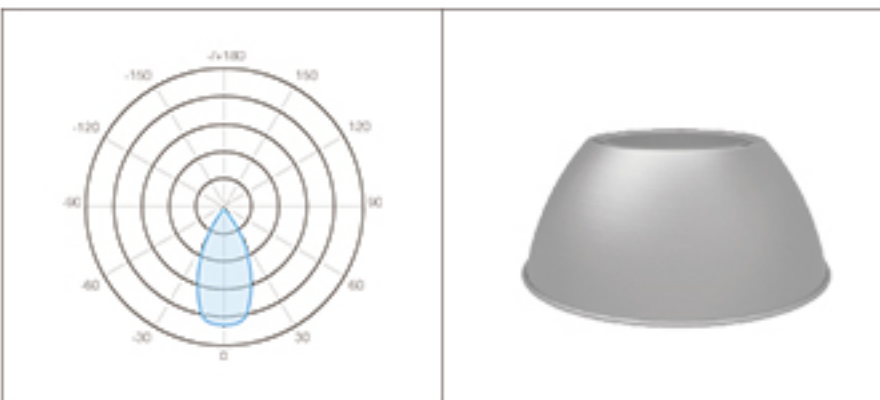
60° Aluminium Reflektor PRE-HB-highlumen-150W-COB-60°R
